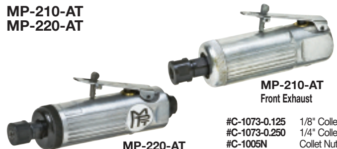
MP-220-AT Rear Exhaust
